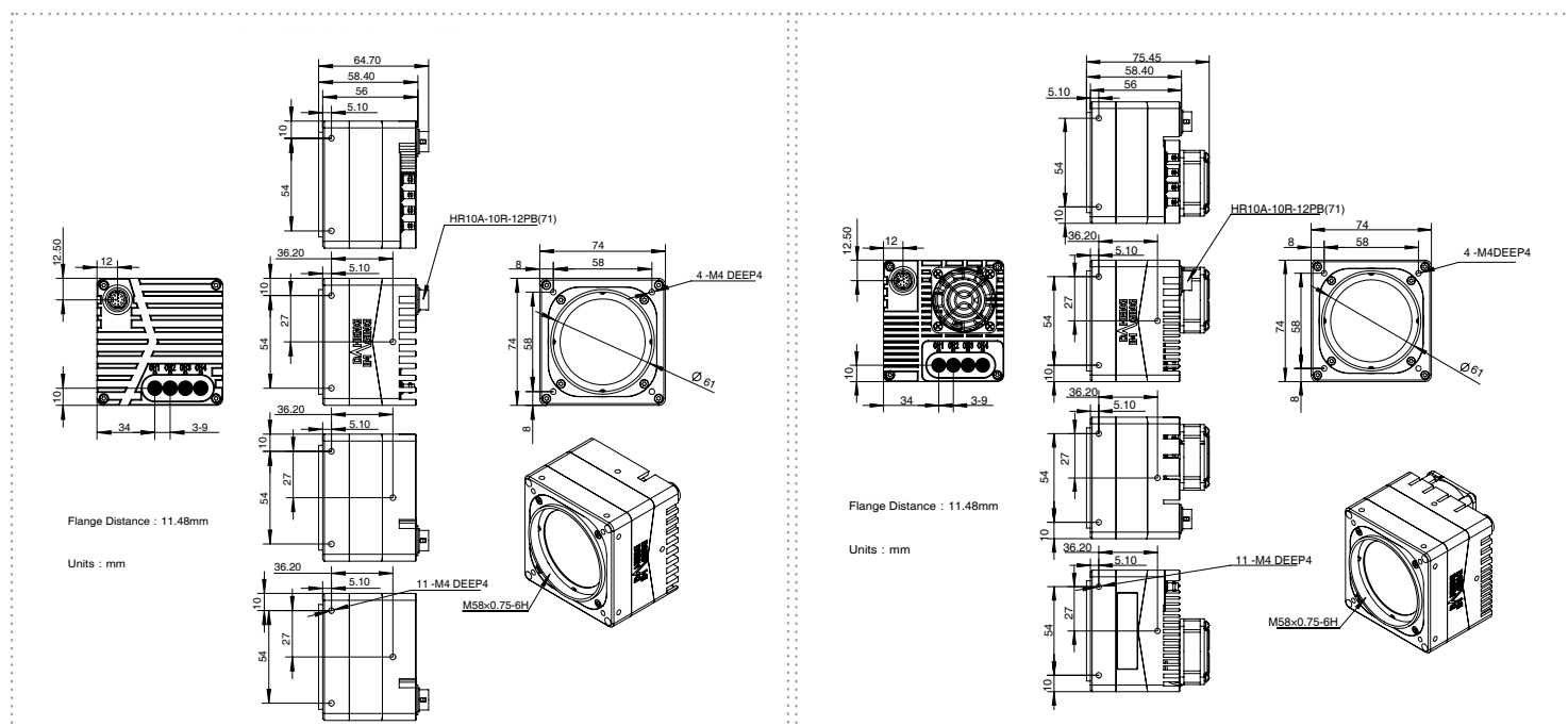
MARS-2626-150X2M/C (M58-mount)
