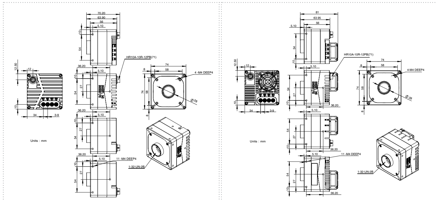
MARS-2626-150X2M/C (C-mount)
