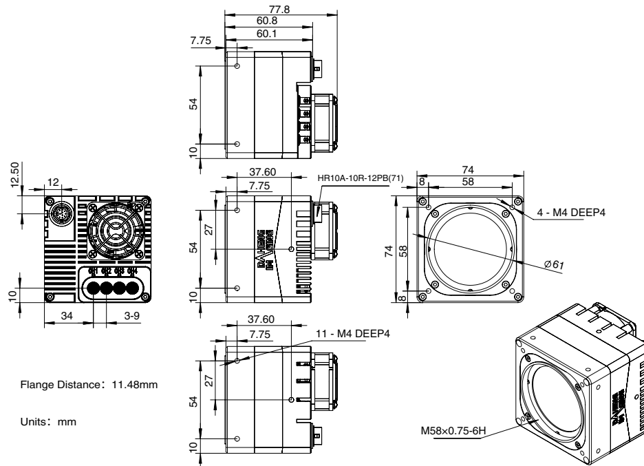
MARS-2100-230X2M/C-NF (M58-mount)
