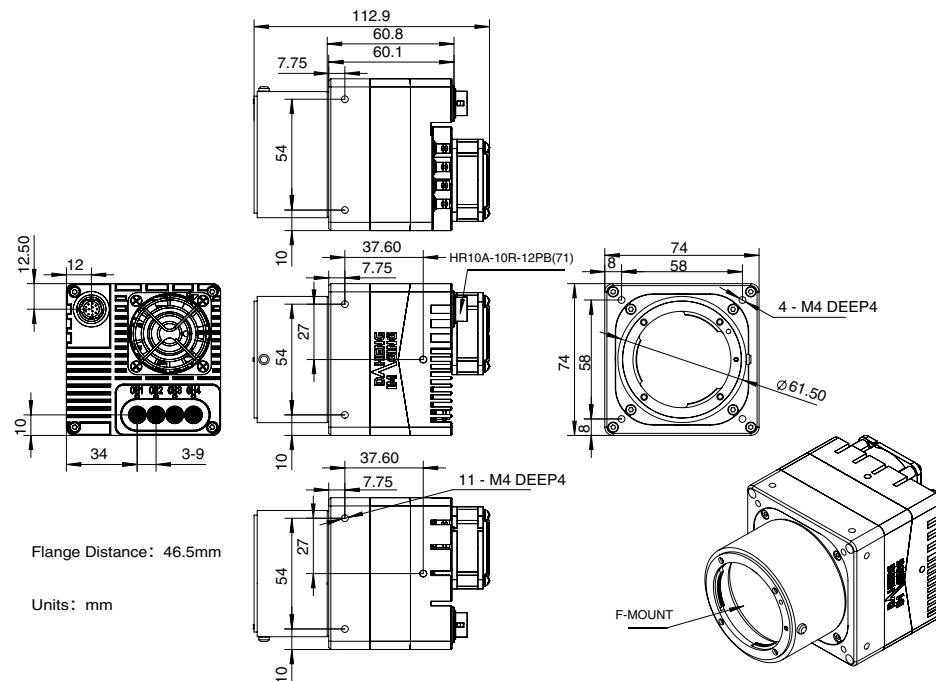
MARS-2100-230X2M/C-NF (F-mount)
